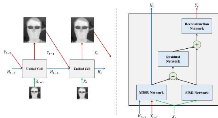
Figure 1: The unrolled recurrent network (left) and components of the unified cell (right) of our super-resolution network.
