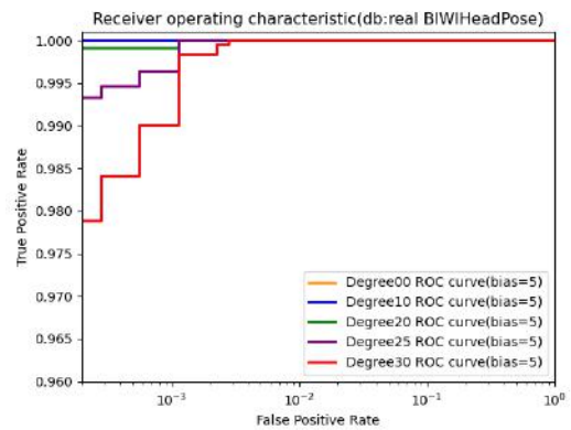
Figure 3: The ROC of real BIWI head pose. Note the classification of various degree in this experiment is only the variation of yaw are selected from BIWI, while pitch and roll are kept at (-5,5).
