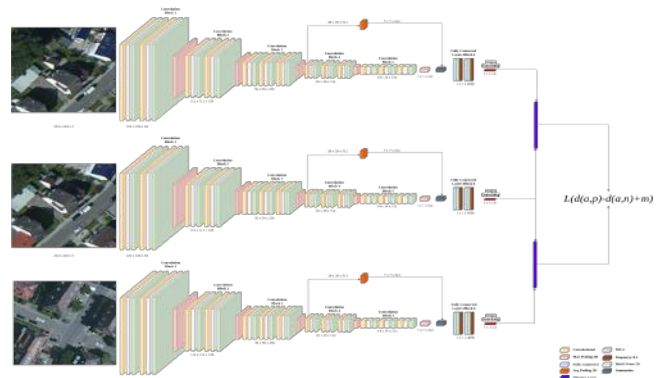
Figure 1: Network architecture visualisation consisting of three modified VGG16 CNN branches (shared weights). Top branch takes as input a positive pair, middle branch takes the anchor satellite image and bottom branch a negative pair image. The outputs are used to calculate the similarity metric between the image pairs.
