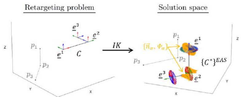
Figure 2: Solution space for mapping/retargeting a kinematic chain to an incongruent hierarchical set of 3D positions.
