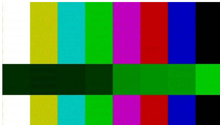
Figure 1: BCI Noise Injection on a Colour Bar Test Pattern
