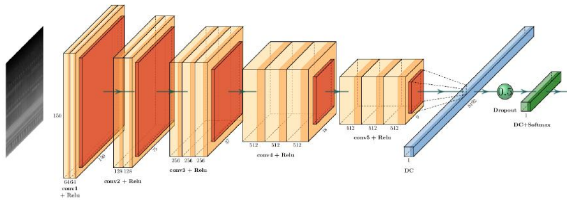
Figure 3: Scheme representing the pretrained VGG16 CNN architecture and the additional layers used to train the model. The convolution, max-pooling and dropout operations are represented in orange, red and green, respectively. Finally, densely connected (DC) layers are added with two activation functions: ReLU before the dropout and softmax afterwards.
