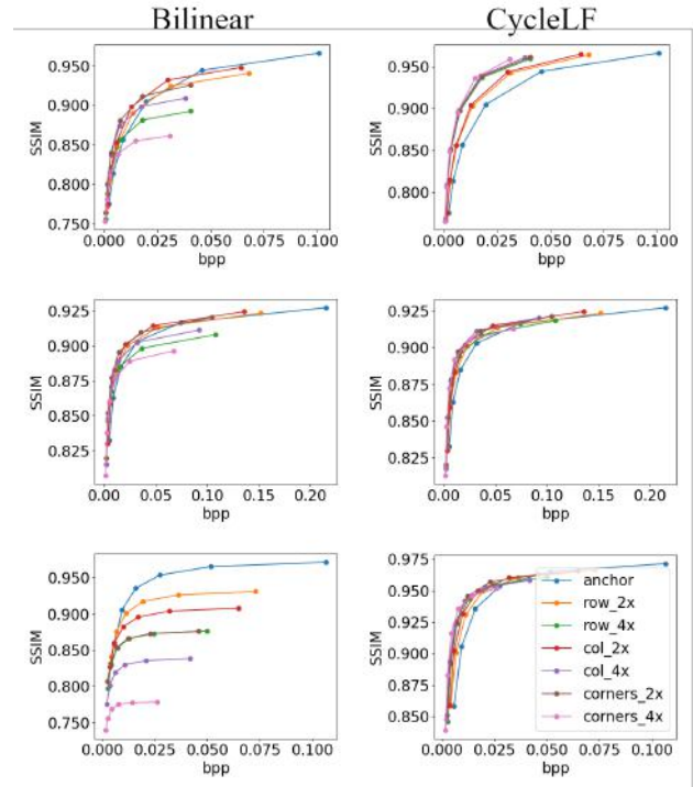
Figure 6: Rate-distortion results as Structural Similarity Index (SSIM) over bit per pixel (bpp). Top row, middle row and bottom row are results on HCI ( Bedroom ), Lytro ( Bee_2 ) and Stanford ( Lego Knights ), respectively.
