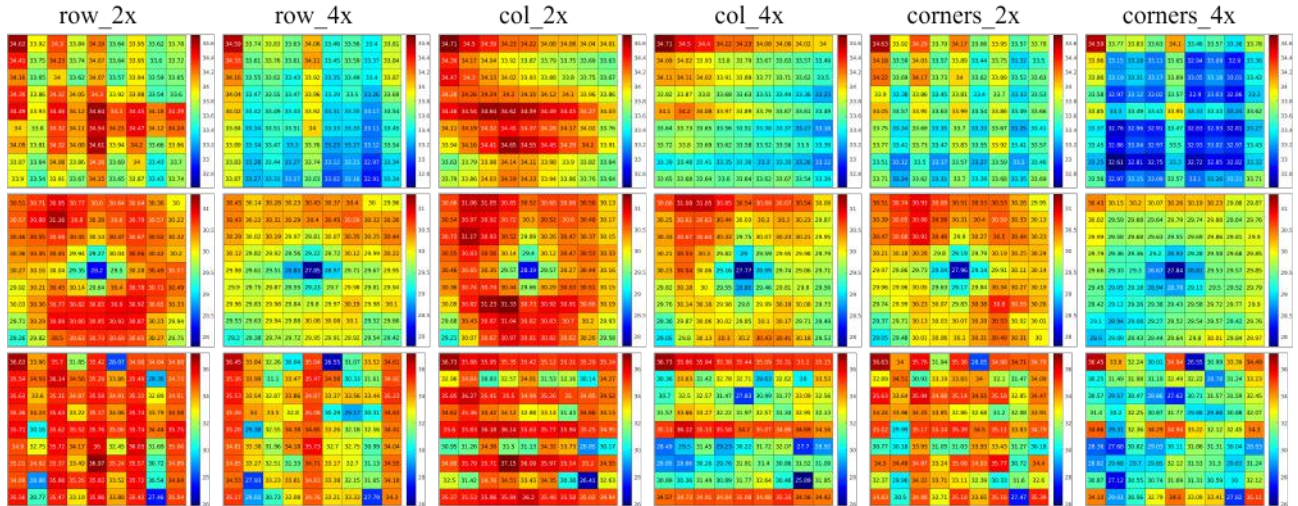
Figure 4: PSNR scores after light field reconstruction with QP = 30 . Top, middle and bottom rows show results from HCI ( Bedroom ), Lytro ( Bee_2 ) and Stanford ( Lego Knights ) datasets using CycleLF [Chen et al., 2020a].
