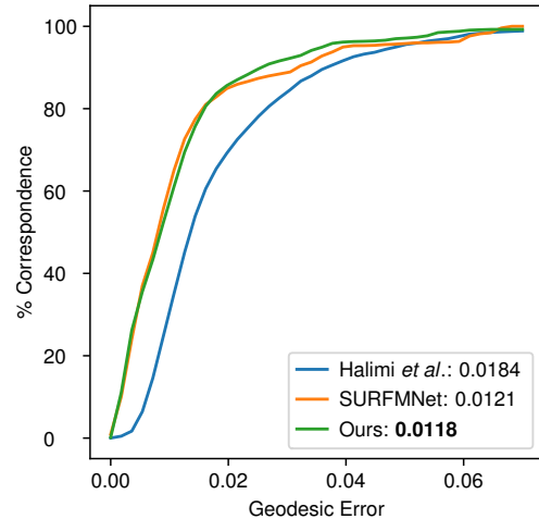
Figure 5: Error evaluation on FAUST dataset compared to [Roufousse and Ovsjanikov, 2018] and [Halimi et al., 2018] on inter-subject and intra-subject pairs. Our multispectral architecture shows improvement even on the near-isometric benchmark.
