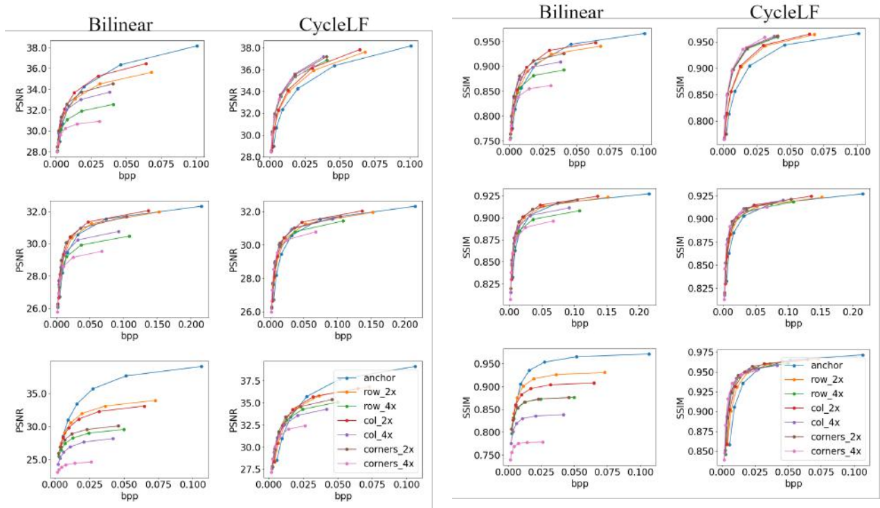
Figure 6: Rate-distortion results as Structural Similarity Index (SSIM) over bit per pixel (bpp). Top row, middle row and bottom row are results on HCI ( Bedroom ), Lytro ( Bee_2 ) and Stanford ( Lego Knights ), respectively.
