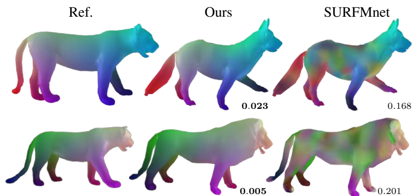
Figure 1: Unsupervised functional maps correspondence between highly non-isometric shapes from the SMAL dataset. Visualization of texture transfer. Mean geodesic error is marked next to each correspondence.
