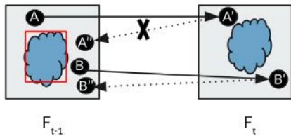
Figure 3: Box and Bidirectional Filters. Bounding box is colored red.
