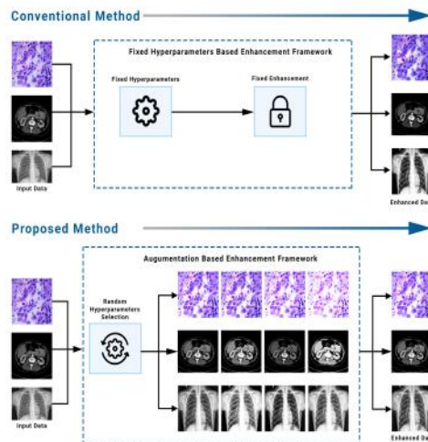
Figure 1: Overview of the proposed random augmentation based enhancement and the conventional enhancement
