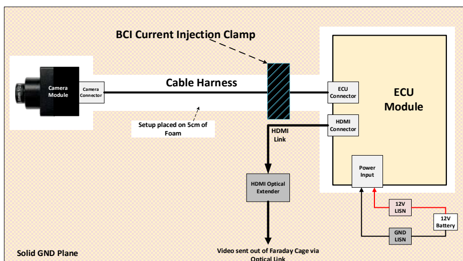
Figure 2: Sample BCI Test Setup for a Single Camera Link
