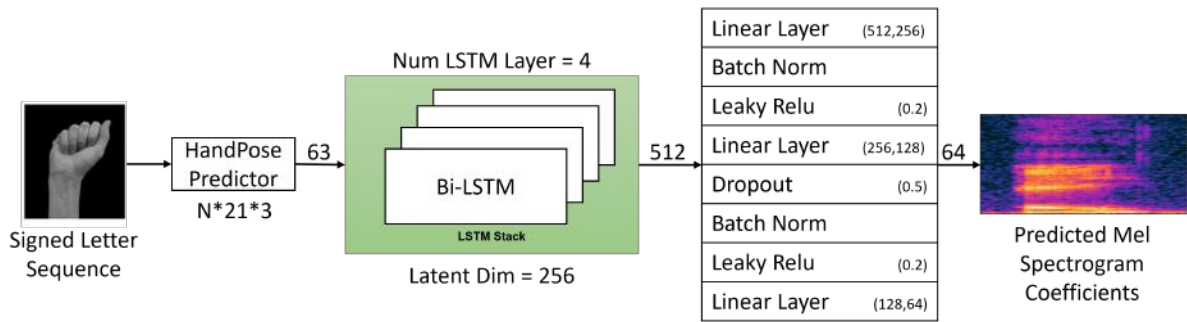
Figure 2: Long Short-Term Memory (LSTM)-based network architecture – The proposed architecture decodes temporal features from and predicts Mel spectrogram coefficients in an autoregressive manner. The keypoints are predicted by an off-the-shelf method.
