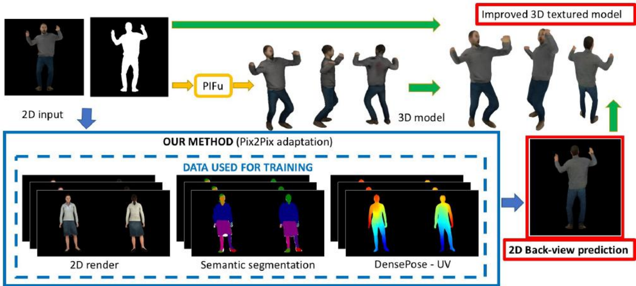
Figure 2: Pipeline overview
